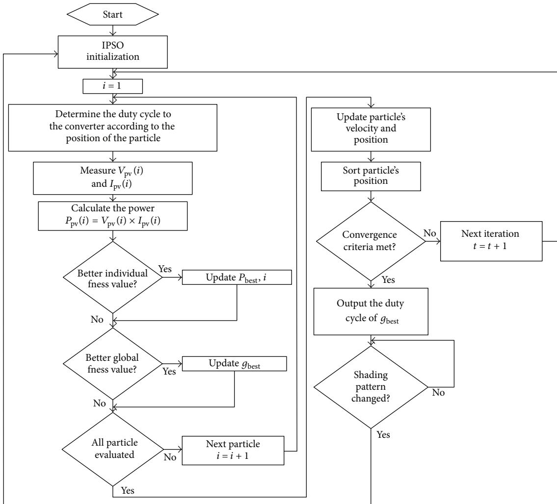
FIGURE 9: Flowchart of IPSO based MPPT algorithm.
