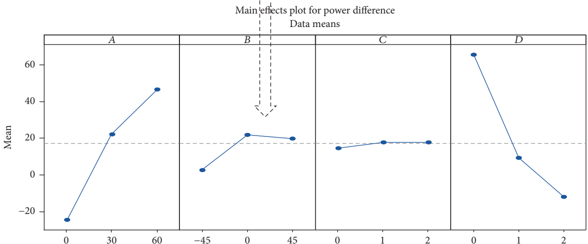
FIGURE 5: Optimum versus main effect inconsistency for factor B: azimuth angle (degrees from south).
