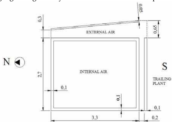
Fig. 2. Cross-section geometry
