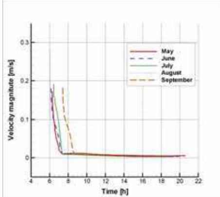
Fig. 21. Daily variation of room average velocities magnitude
