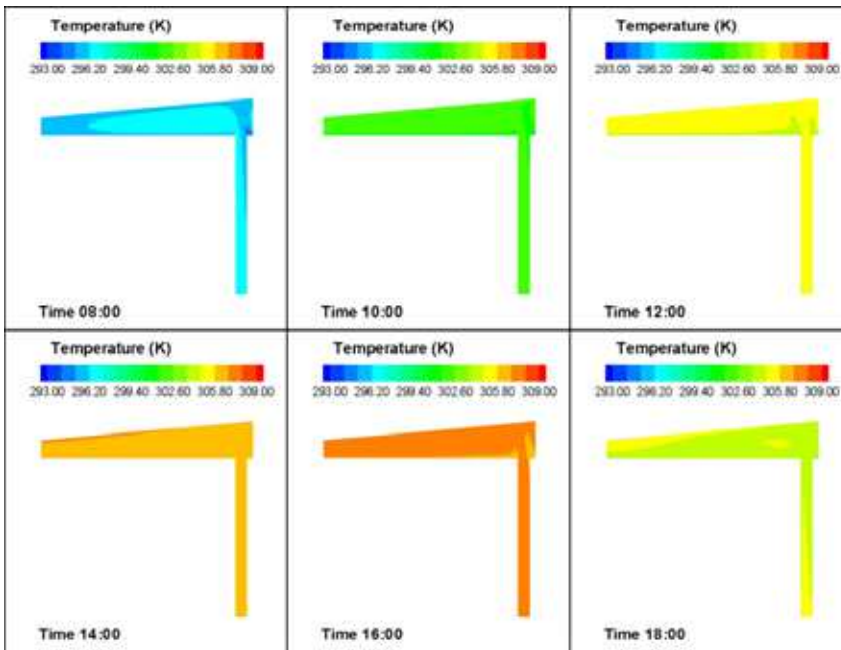
Fig. 8. Temperature iso-contours around the test cell
