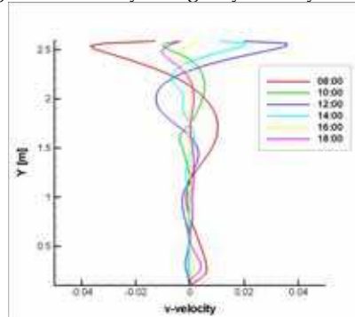
Fig. 16. v -velocity along y -symmetry axes
