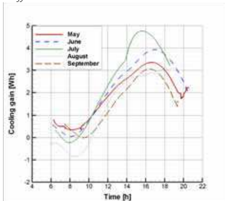
Fig. 23. Daily variation of cooling load reduction
