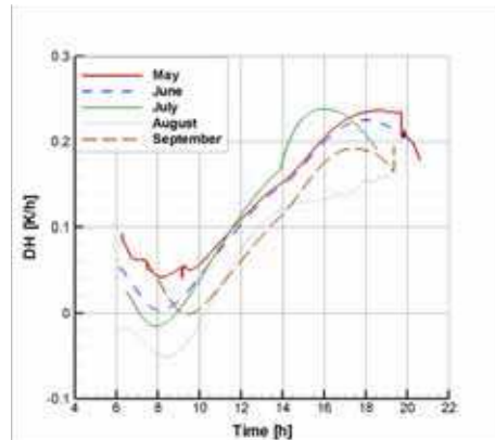
Fig. 24 Daily variation of degree hours
