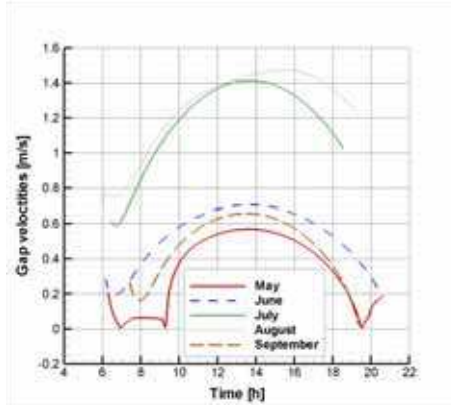
Fig. 22. Daily variation of gap average velocities magnitude
