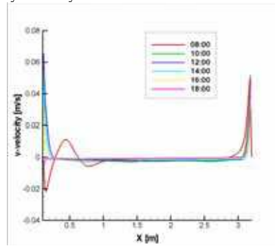
Fig. 14. v -velocity along x -symmetry axes
